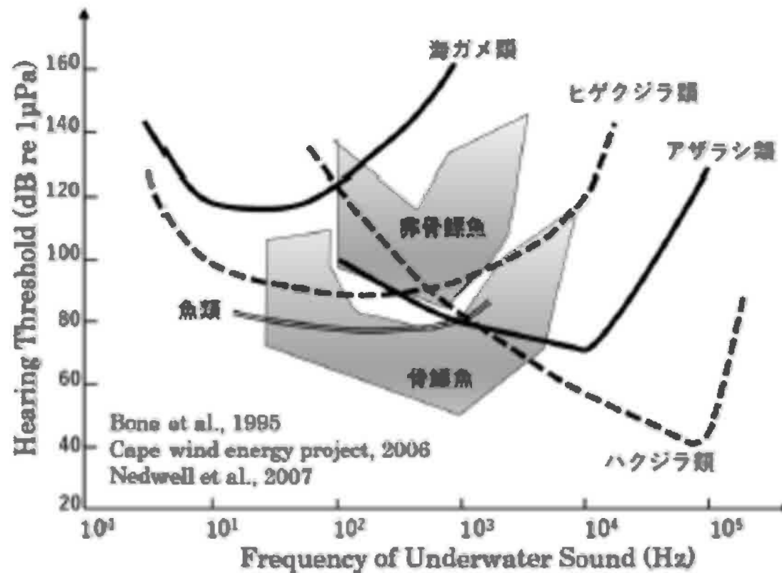
Fig. 4 Audiogram of marine organisms.
